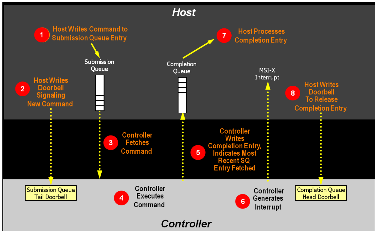
Figure 8: Command Processing
