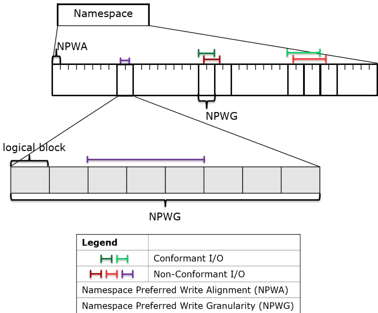
Figure 144: Example namespace broken down to illustrate potential NPWA and NPWG settings
