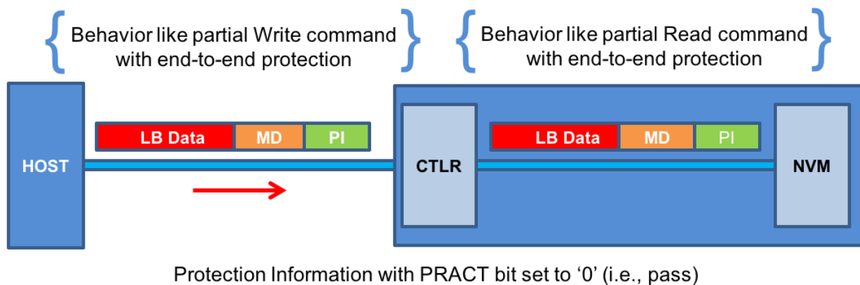
Figure 135: Protection Information Processing for Compare
