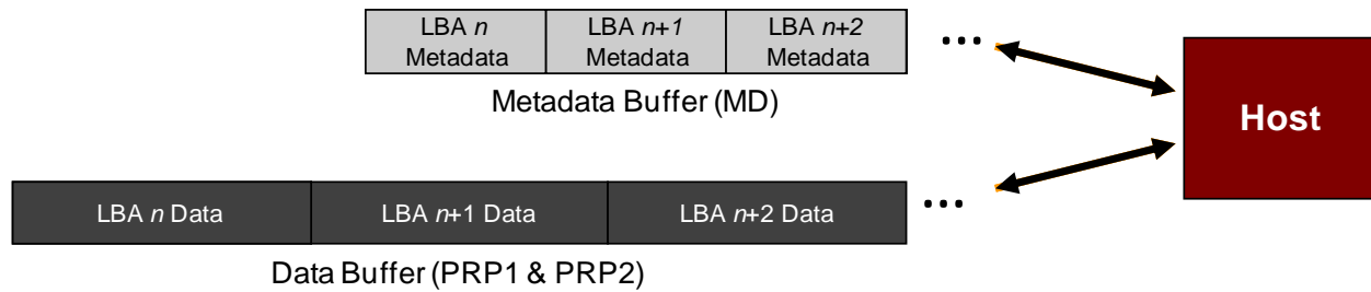
Figure 150: Metadata – Transferred as Separate Buffer
