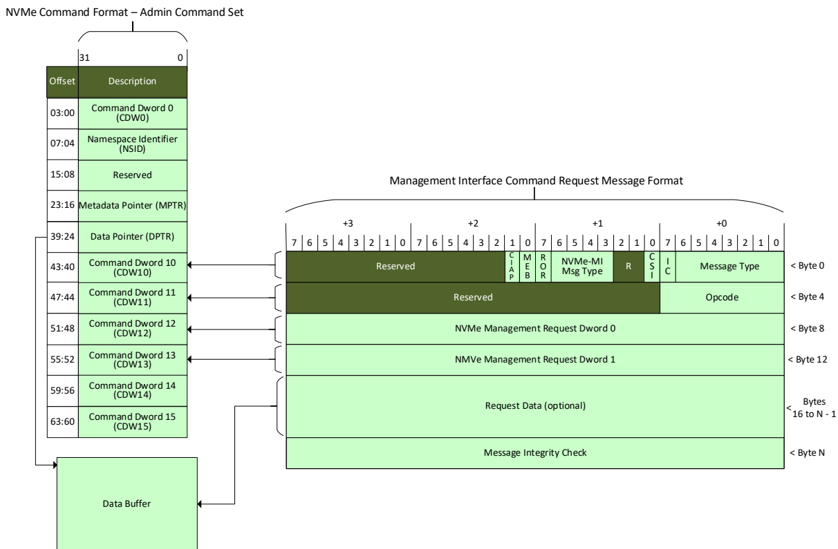
Figure 46: NVMe-MI Send Command Request Message to NVMe Admin Command SQE Mapping Diagram
