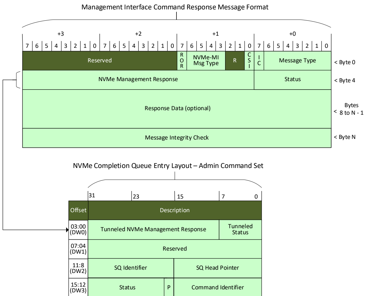
Figure 49: NVMe-MI Send Command Response Message to NVMe Admin Command CQE Mapping Table
