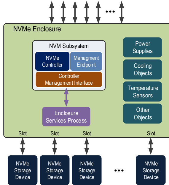
Figure 9: Example NVMe Enclosure
