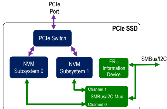
Figure 8: NVMe Storage Device with two NVMe Subsystems and an SMBus/I2C Mux
