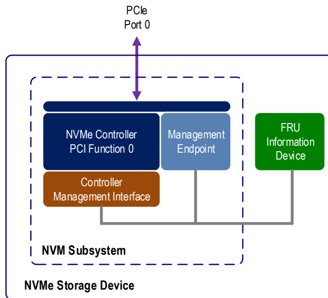
Figure 5: Single-Port PCIe SSD
