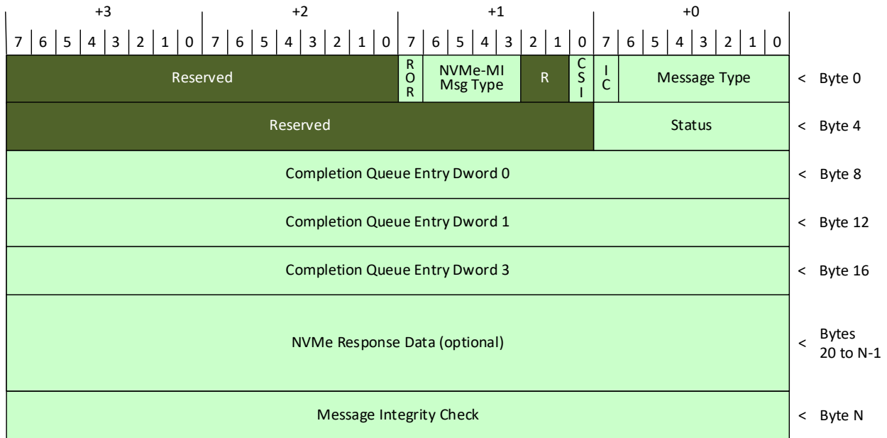
Figure 120: NVMe Admin Command Response Description
