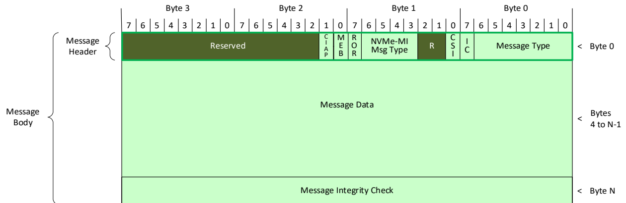
Figure 18: NVMe-MI Message
