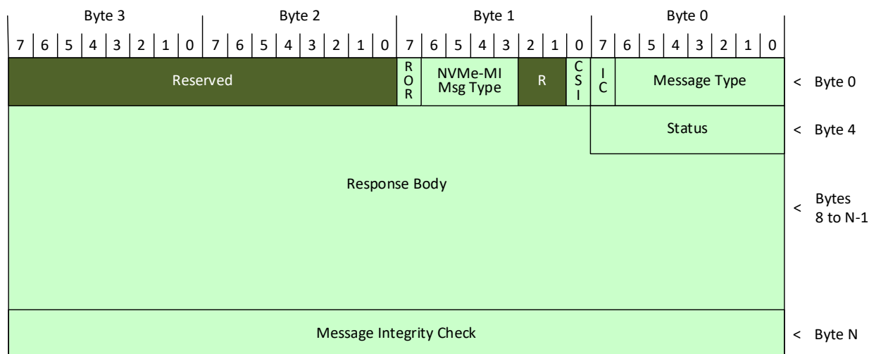
Figure 26: Response Message Format
