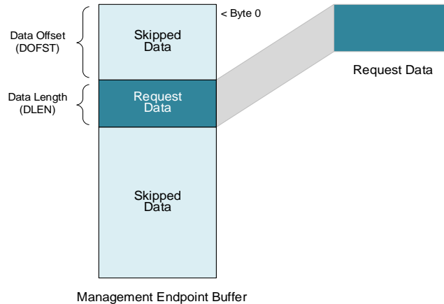
Figure 87: Management Endpoint Buffer Write Request Data
