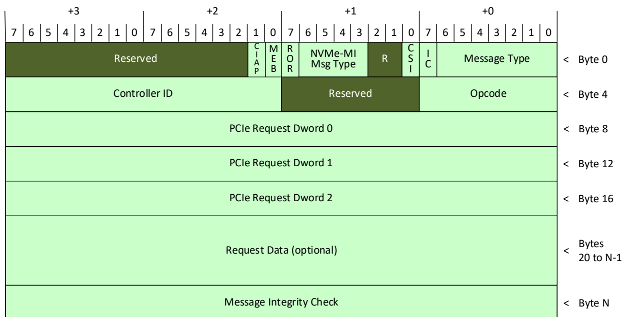
Figure 128: PCIe Command Request Format
