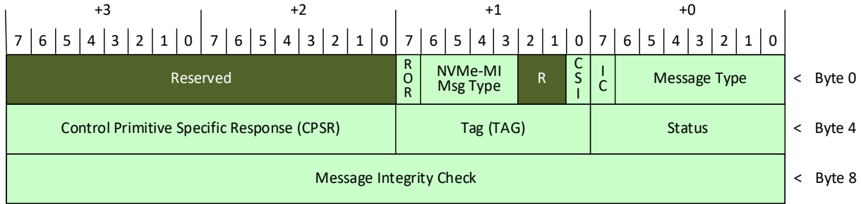
Figure 39: Control Primitive Success Response Fields
