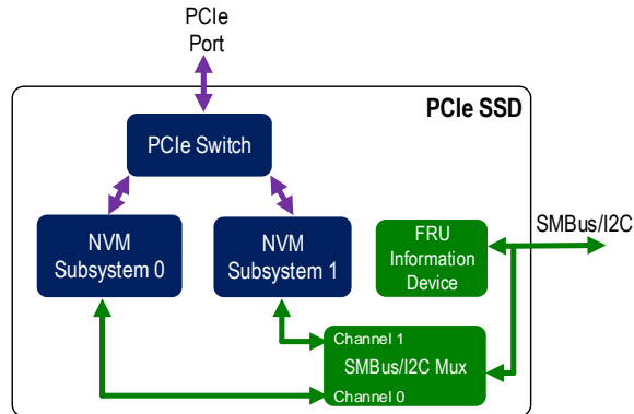
Figure 8: NVMe Storage Device with two NVM Subsystems and an SMBus/I2C Mux
