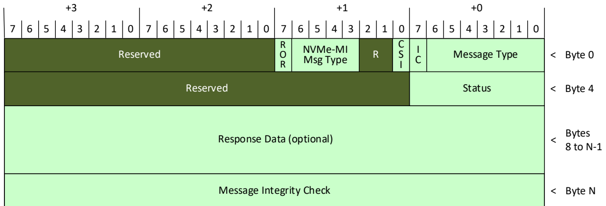
Figure 132: PCIe Command Response Description
