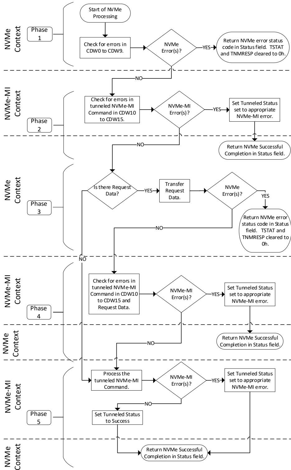
Figure 51: NVMe-MI Send Command Servicing Model
