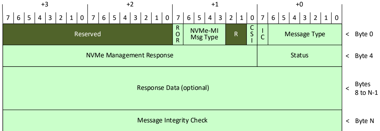
Figure 63: NVMe-MI Command Response Message Description (NCRESP)
