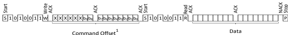
Figure 149: I2C Read from a FRU Information Device
