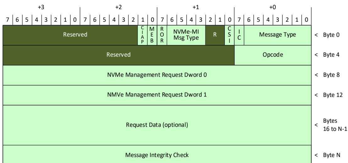
Figure 57: NVMe-MI Command Request Message Format
