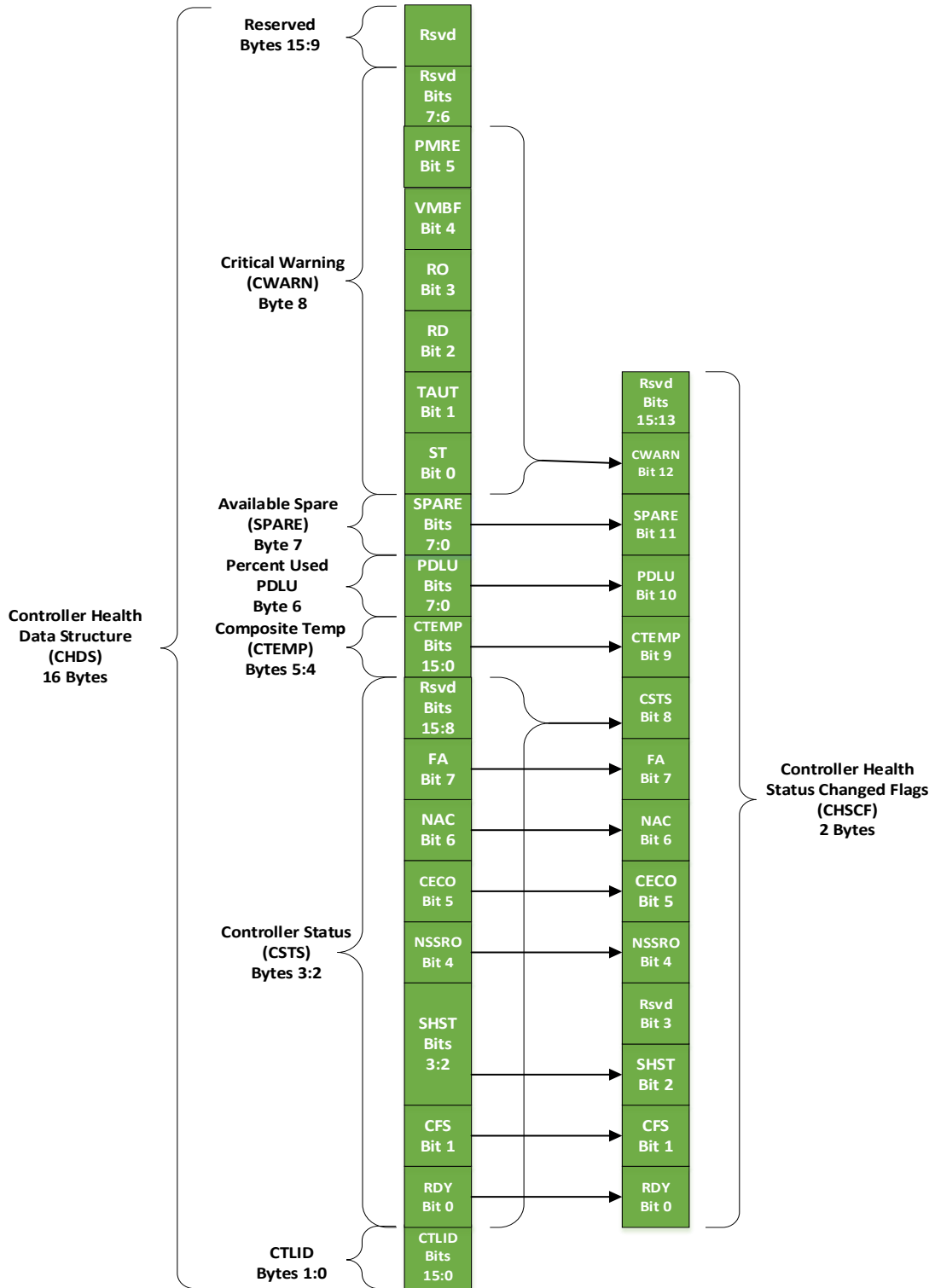
Figure 83: Controller Health Data Structure to Controller Health Status Changed Flags Mapping
