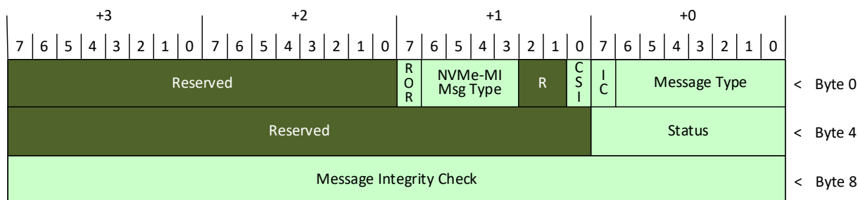
Figure 29: Generic Error Response
