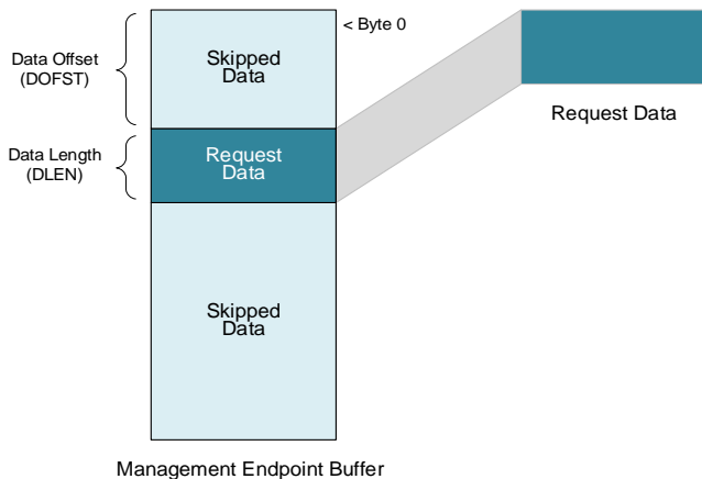
Figure 87: Management Endpoint Buffer Write Request Data
