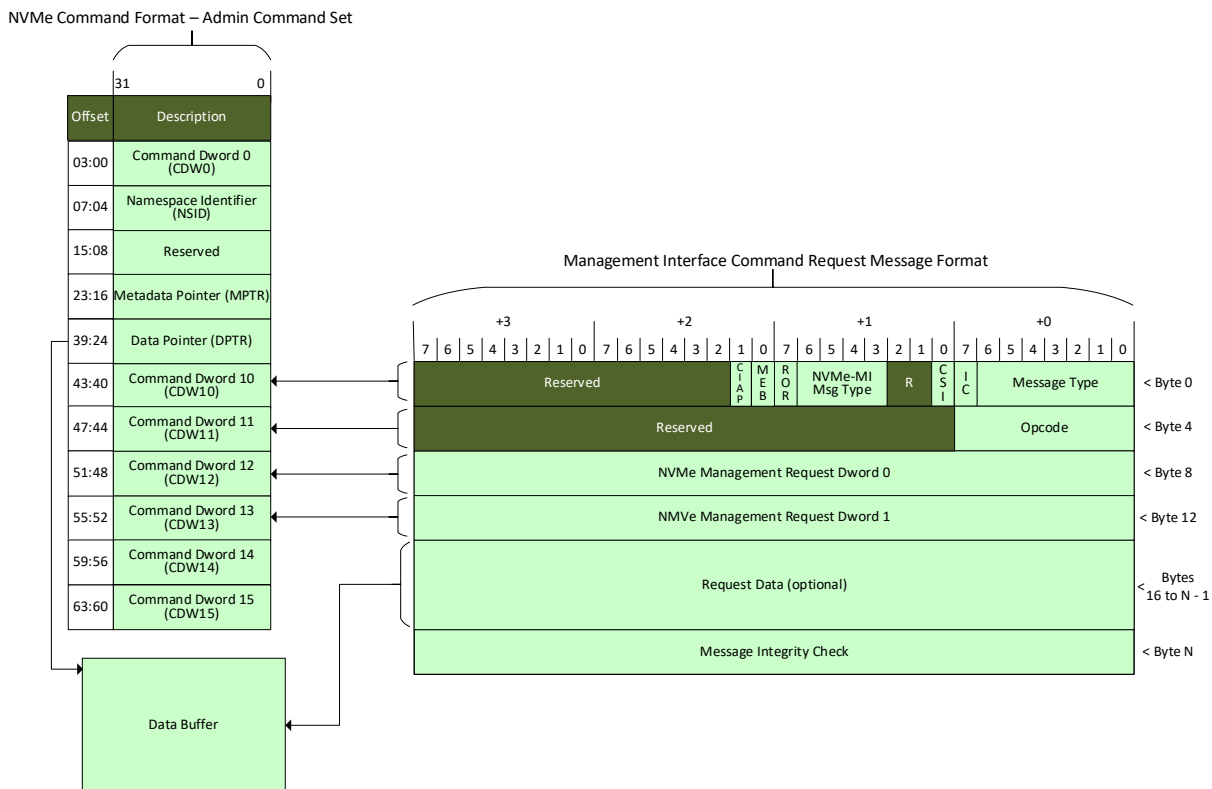
Figure 46: NVMe-MI Send Command Request Message to NVMe Admin Command SQE Mapping Diagram
