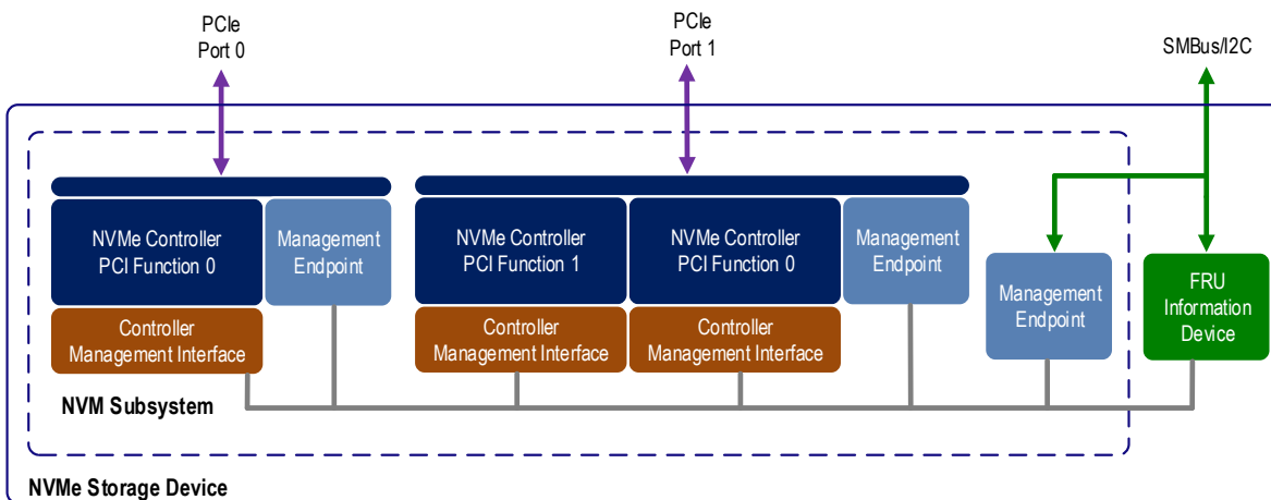
Figure 6: Dual-Port PCIe SSD with SMBus/I2C
