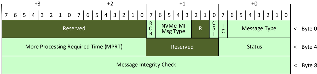
Figure 32: More Processing Required Response
