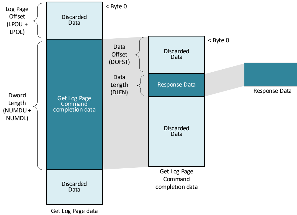
Figure 122: NVMe Get Log Page Command Response Data Example
