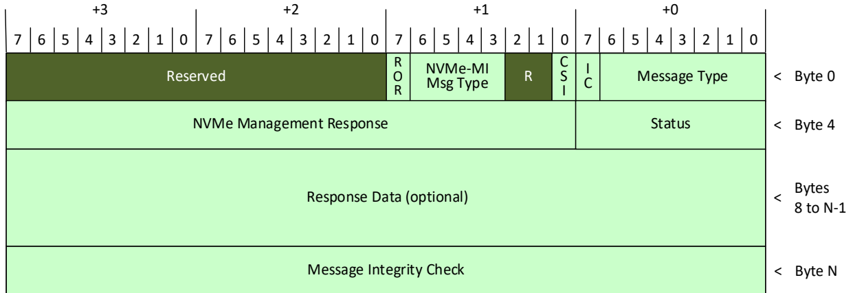
Figure 62: NVMe-MI Command Response Message Format
