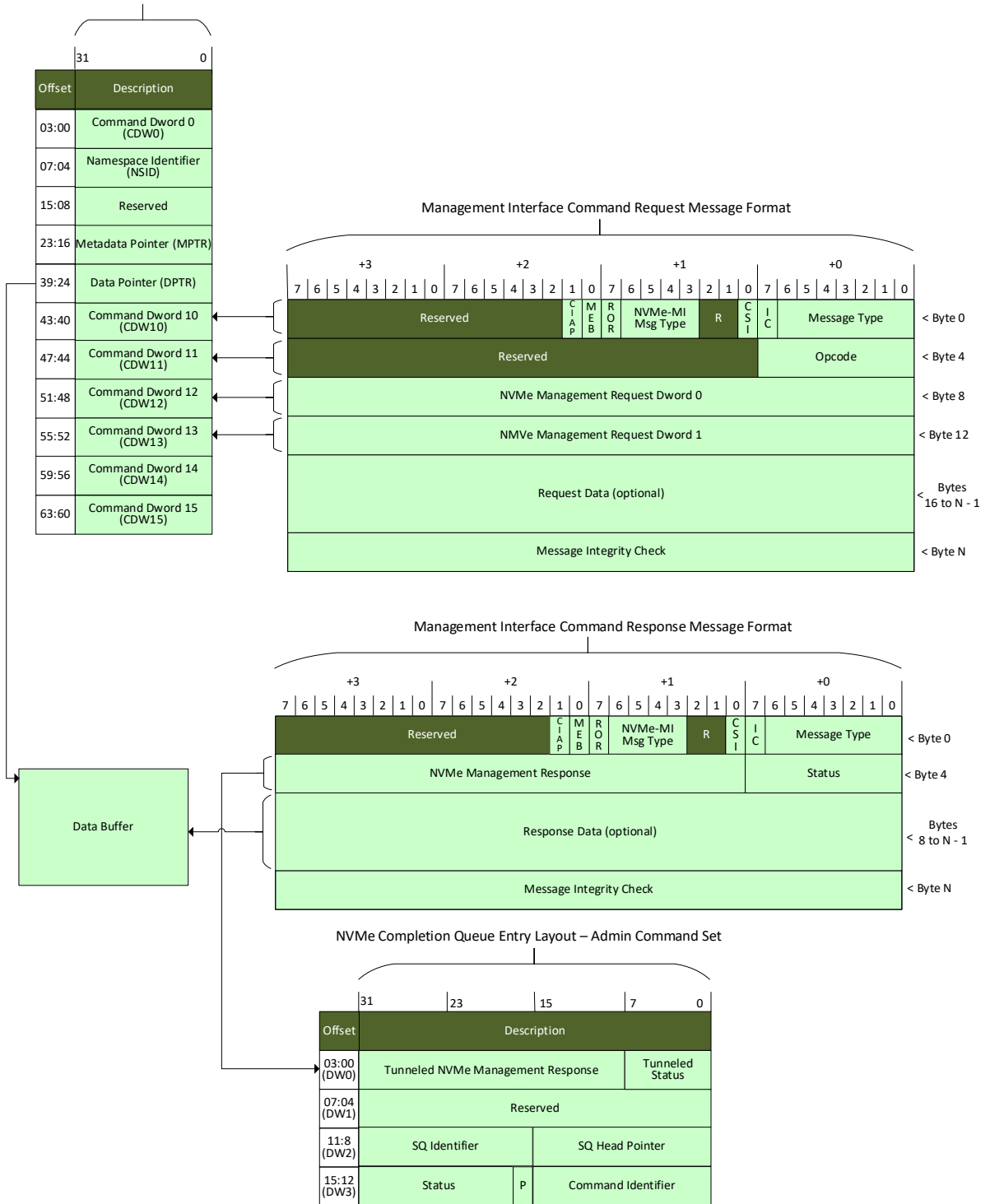
Figure 52: NVMe-MI Receive Command Request/Response Message to NVMe Admin Command SQE/CQE Mapping Diagram
