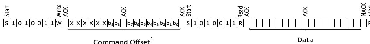
Figure 149: I2C Read from a FRU Information Device
