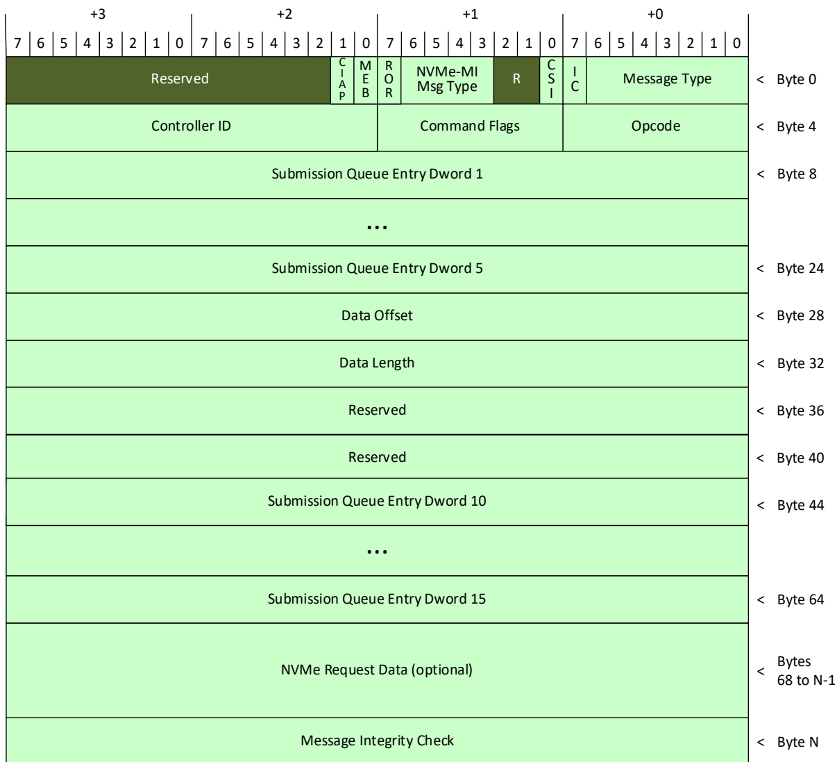
Figure 118: NVMe Admin Command Request Description
