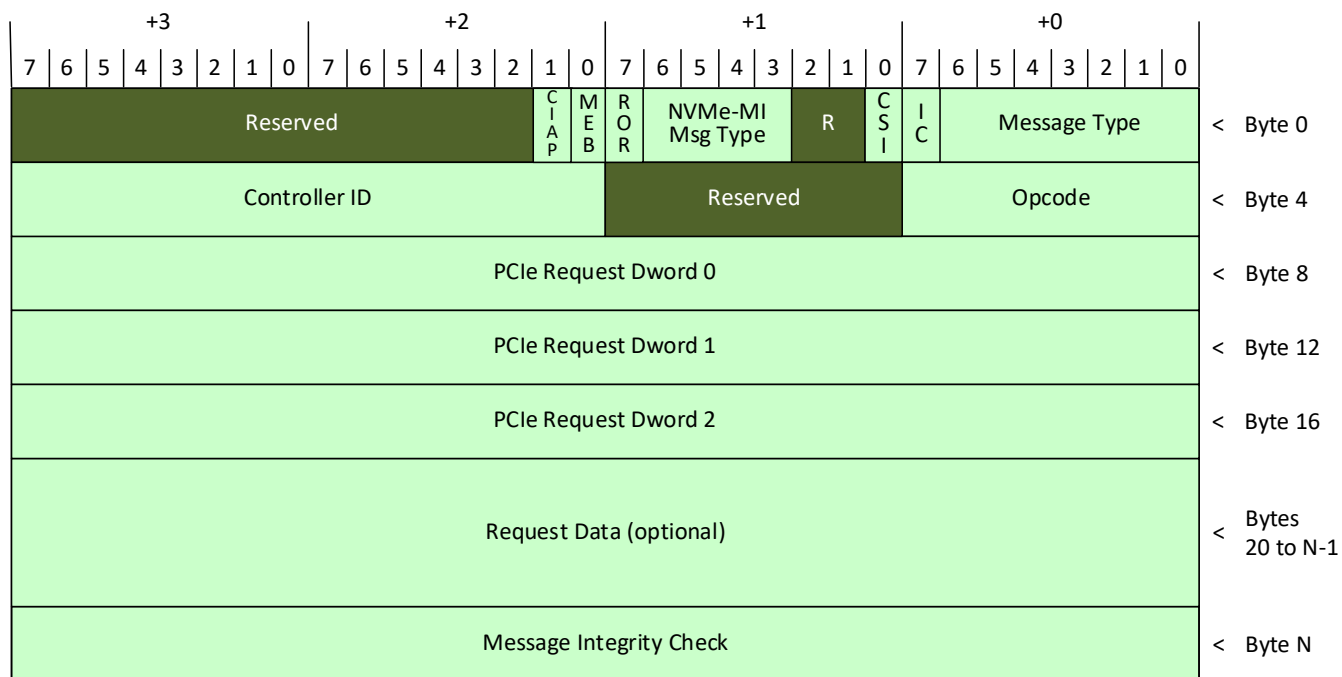
Figure 128: PCIe Command Request Format
