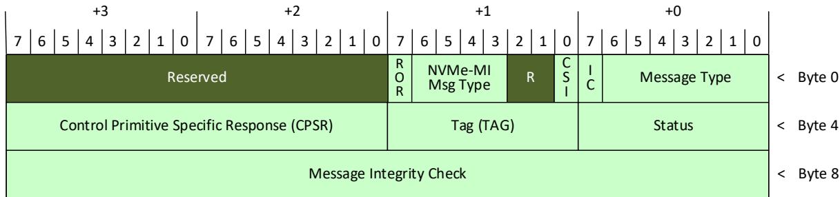
Figure 38: Control Primitive Success Response Format
