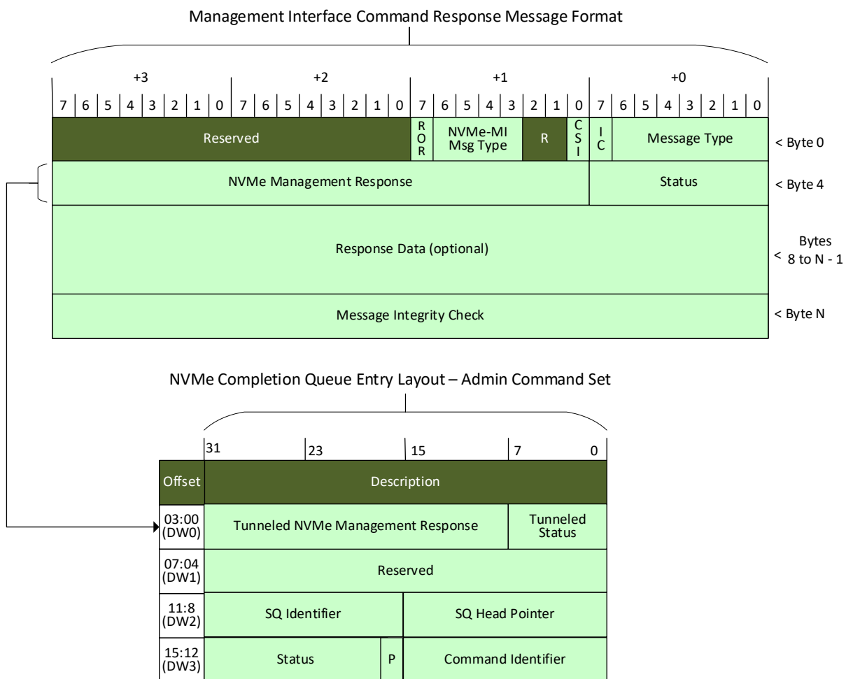
Figure 48: NVMe-MI Send Command Response Message to NVMe Admin Command CQE Mapping Diagram
