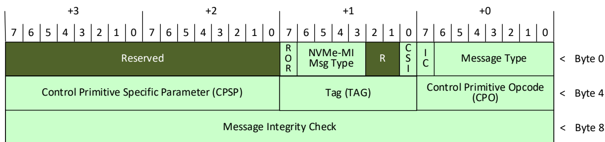
Figure 35: Control Primitive Request Message Format
