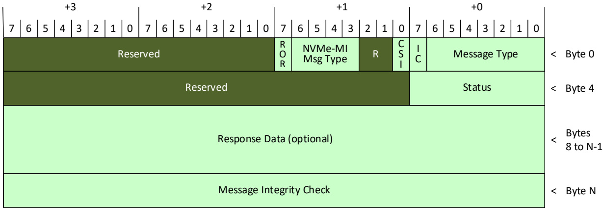
Figure 131: PCIe Command Response Format
