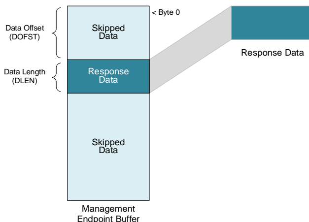
Figure 84: Management Endpoint Buffer Read Response Data
