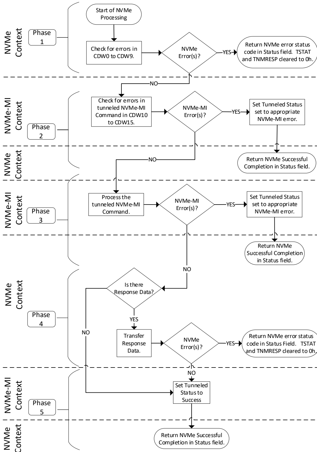
Figure 56: NVMe-MI Receive Command Servicing Model
