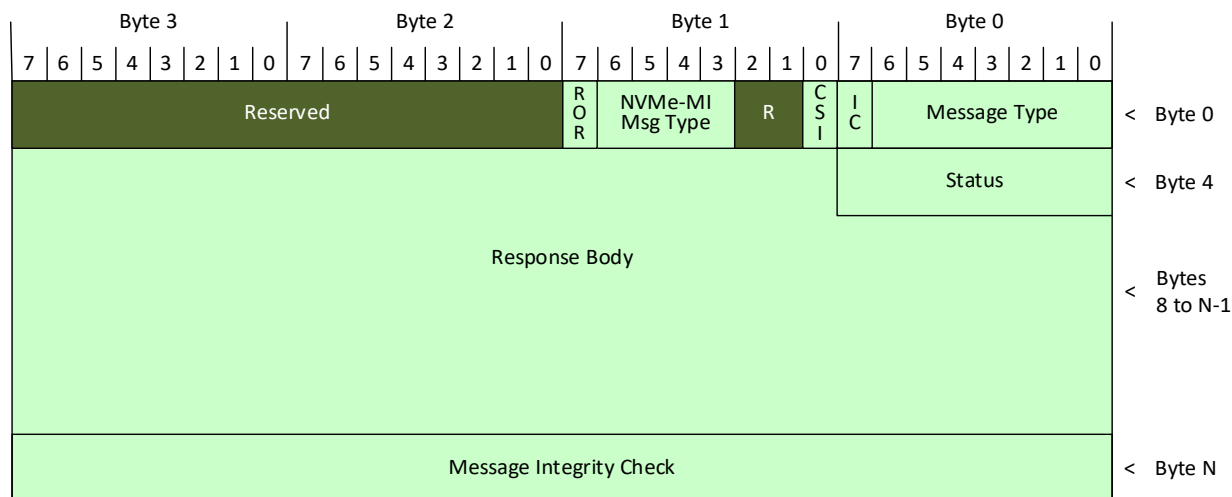
Figure 26: Response Message Format
