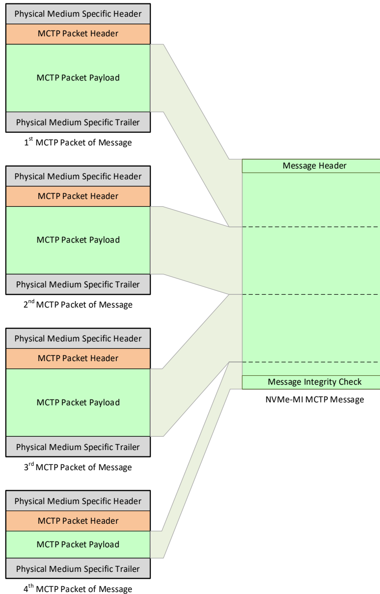
Figure 24: NVMe-MI Message Spanning Multiple MCTP Packets
