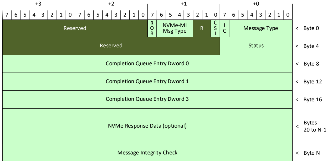
Figure 119: NVMe Admin Command Response Format
