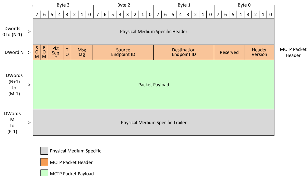
Figure 22: MCTP Packet Format
