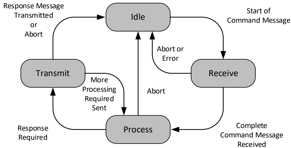
Figure 34: Command Servicing State Diagram
